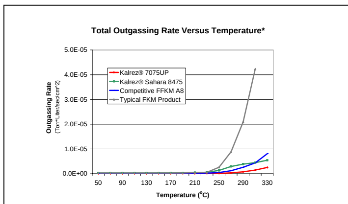
Figure 3. Total Outgassing Rate versus Temperature
